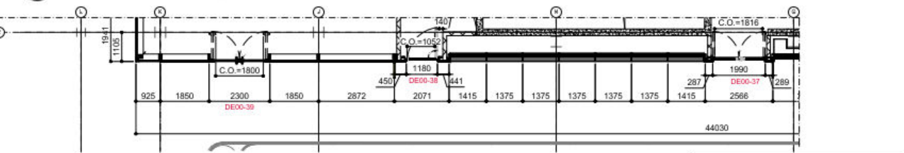
3A LOWER GROUND PLAN 1:150
